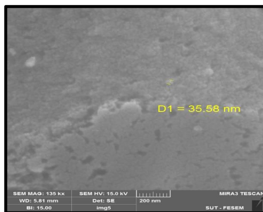
Figure 4: SEM image of the prepared activated carbon at a magnification of 200 nm
