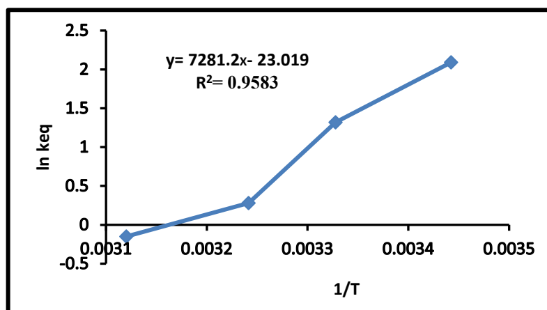
Figure (8): Decrease in Adsorption Efficiency with Increasing Temperature for Chlorpheniramine
