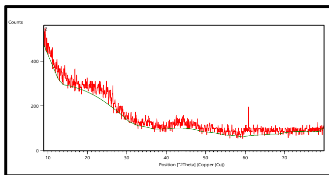
Figure 2: XRD pattern of the synthesized activated carbon.
